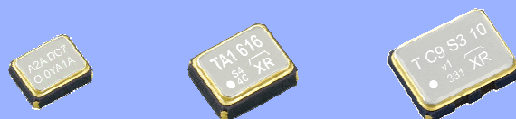
TG-5006CJ (2.0 × 1.6 × 0.73 mm) TG-5006CG (2.5 × 2.0 × 0.8 mm) TG-5006CE (3.2 × 2.5 × 0.9 mm)
