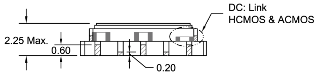
FRONT VIEW (DC)
